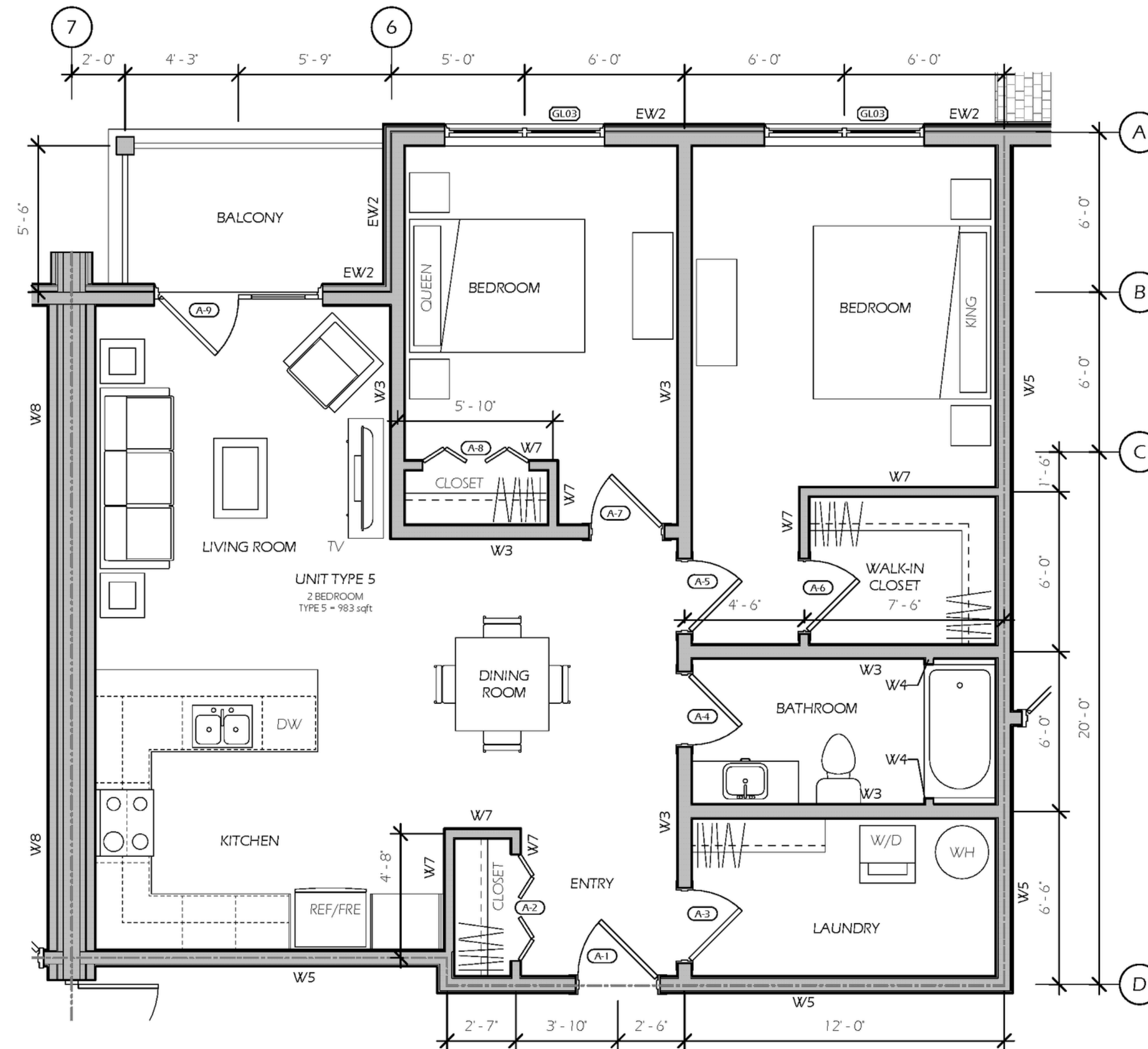
1 UNIT TYPE 5 ENLARGEMENT A105 1/4" = 1'-0"
