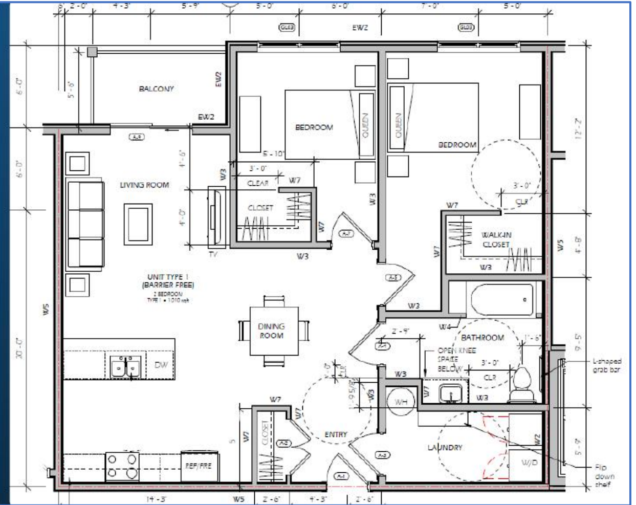
2-Bedroom, 1 Bathroom | 1,010 sqft. Barrier-Free & Accessible
