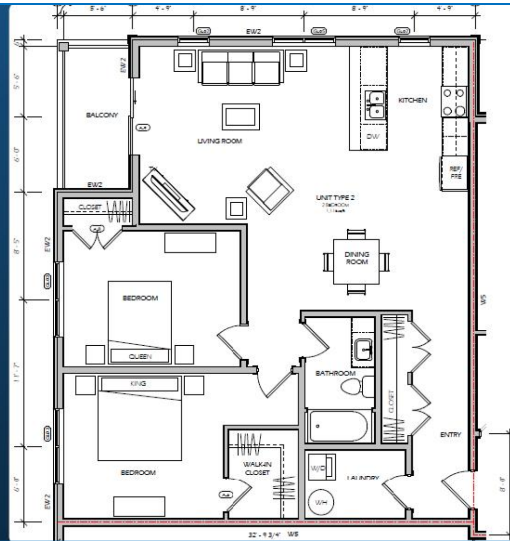
2-Bedroom, 1 Bathroom | 1,116 sqft.
